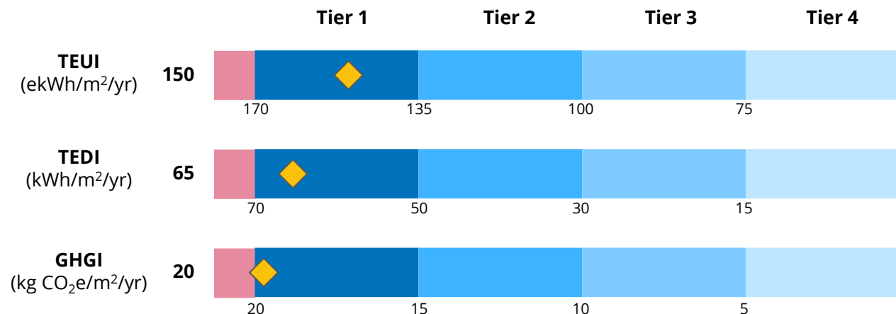
Figure 5: Baseline Performance Package Results
