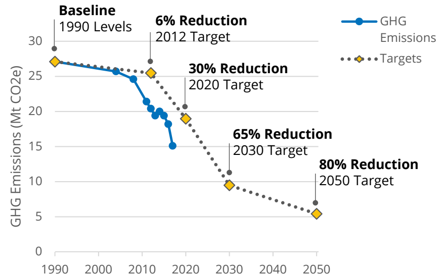
Figure 3: City of Toronto GHG Emissions and Targets
