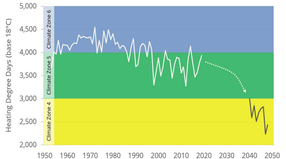
Figure 14: Historical and Forecasted Heating Degree Days at Toronto Pearson International Airport
