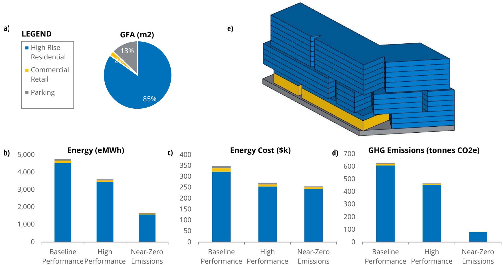
Figure 9: a) Breakdown of Development Site Gross Floor Area by Archetype, b) Energy Results, c) Energy Cost Results, d) GHG Emissions Results, e) Modelled Geometry by Archetype
