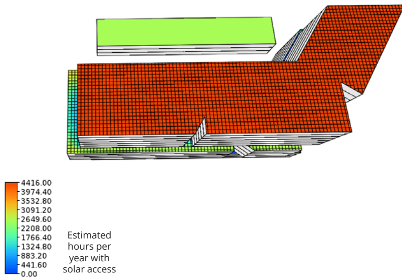
PV Suitability Analysis
