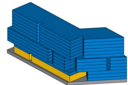
Figure 4 (b): Project Geometry with Modelled Archetypes (NE View)
