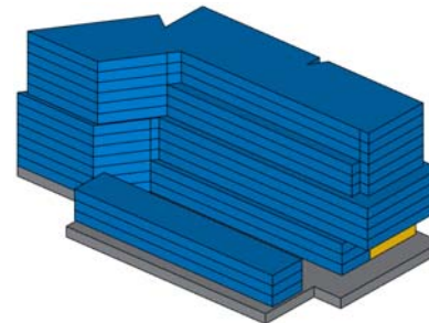
Figure 4 (a): Project Geometry with Modelled Archetypes (SW View)
