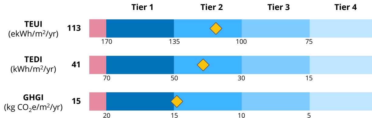
Figure 6: High Performance Package Results
