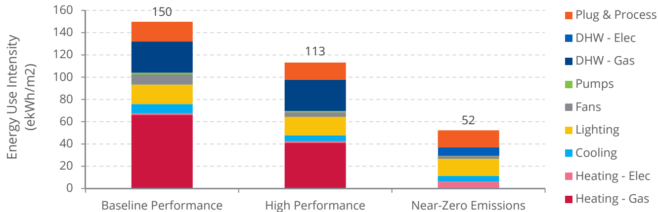
Figure 8: Energy End-Use Breakdown
