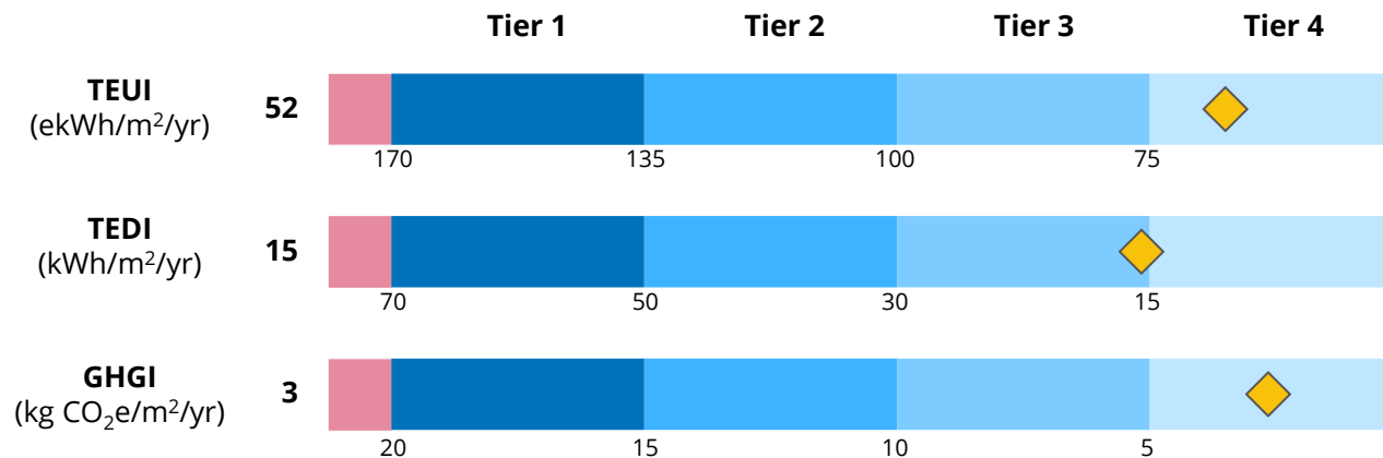
Figure 7: Near-Zero Emissions Package Results
